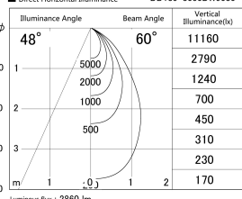
■ Direct Horizontal Illuminance DD139-3050DW9030
