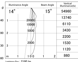
■ Direct Horizontal Illuminance DD139-2015DW9035
