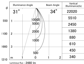
■ Direct Horizontal Illuminance DD139-2530DW9035
