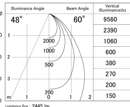
■ Direct Horizontal Illuminance DD139-2550DW9035
