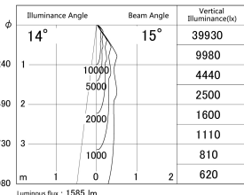
■ Direct Horizontal Illuminance DD139-1515DW9040
