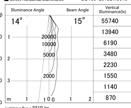
■ Direct Horizontal Illuminance DD139-2015DW9040
