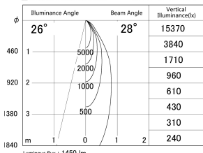
■ Direct Horizontal Illuminance DD139-1520DB9027
