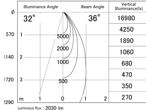
■ Direct Horizontal Illuminance DD139-2030DB9027
