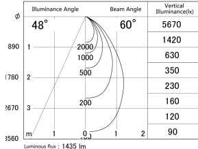
■ Direct Horizontal Illuminance DD139-1550DB9030
