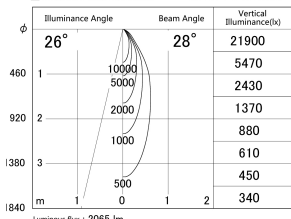
■ Direct Horizontal Illuminance DD139-2020DB9030
