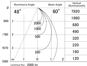
■ Direct Horizontal Illuminance DD139-2050DB9030
