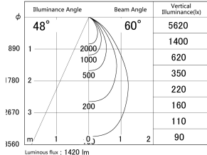
■ Direct Horizontal Illuminance DD139-1550DB9035
