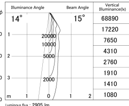
■ Direct Horizontal Illuminance DD139-3015DB9035
