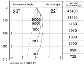
■ Direct Horizontal Illuminance DD139-3020DB9035
