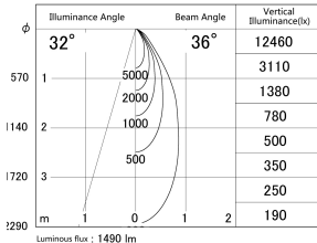
■ Direct Horizontal Illuminance DD139-1530DB9040
