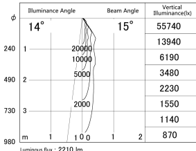
■ Direct Horizontal Illuminance DD139-2015DB9040
