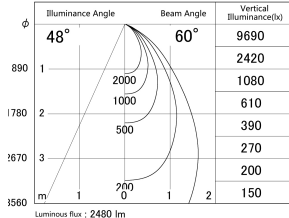
■ Direct Horizontal Illuminance DD139-2550DB9040
