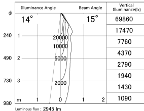
■ Direct Horizontal Illuminance DD139-3015DB9040
