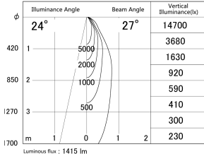
■ Direct Horizontal Illuminance DD139-1520WW9027
