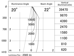
■ Direct Horizontal Illuminance DD139-2520WW9027
