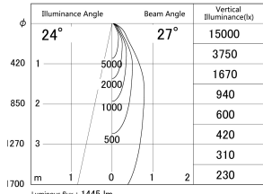
■ Direct Horizontal Illuminance DD139-1520WW9030
