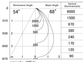
■ Direct Horizontal Illuminance DD139-2050WW9030
