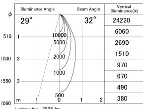
■ Direct Horizontal Illuminance DD139-3030WW9030
