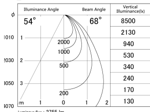
■ Direct Horizontal Illuminance DD139-3050WW9030
