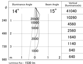
■ Direct Horizontal Illuminance DD139-1515WW9035
