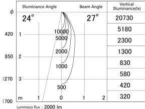
■ Direct Horizontal Illuminance DD139-2020WW9035
