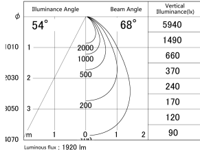
■ Direct Horizontal Illuminance DD139-2050WW9035
