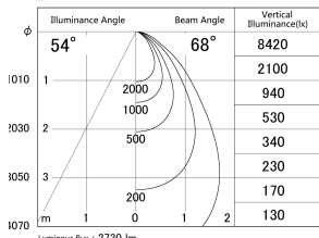
■ Direct Horizontal Illuminance DD139-3050WW9035
