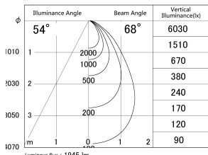
■ Direct Horizontal Illuminance DD139-2050WW9040
