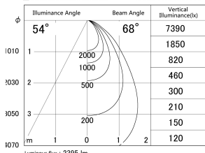
■ Direct Horizontal Illuminance DD139-2550WW9040
