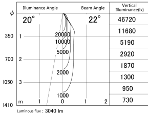
■ Direct Horizontal Illuminance DD139-3020WW9040
