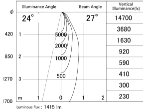
■ Direct Horizontal Illuminance DD139-1520WB9027
