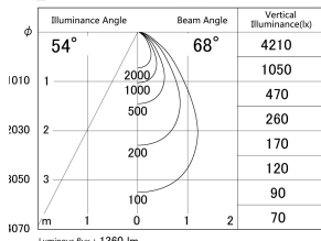
■ Direct Horizontal Illuminance DD139-1550WB9027
