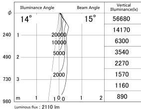
■ Direct Horizontal Illuminance DD139-2015WB9027
