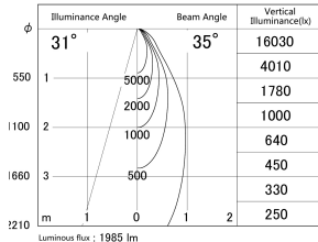
■ Direct Horizontal Illuminance DD139-2030WB9027
