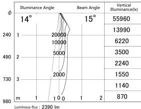
■ Direct Horizontal Illuminance DD139-2515WB9027
