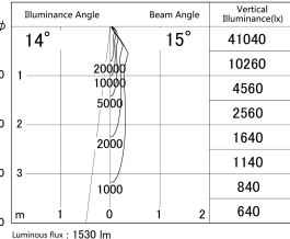
■ Direct Horizontal Illuminance DD139-1515WB9035
