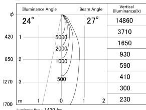
■ Direct Horizontal Illuminance DD139-1520WB9035
