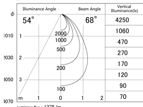
■ Direct Horizontal Illuminance DD139-1550WB9035
