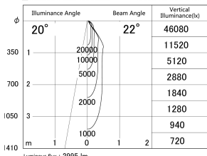
■ Direct Horizontal Illuminance DD139-3020WB9035
