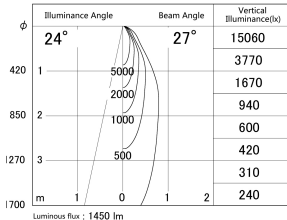
■ Direct Horizontal Illuminance DD139-1520WB9040
