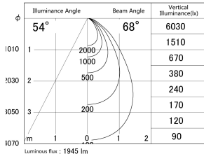
■ Direct Horizontal Illuminance DD139-2050WB9040
