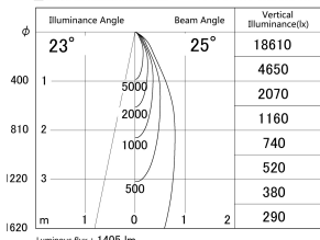
■ Direct Horizontal Illuminance DD139-1520MW9027D
