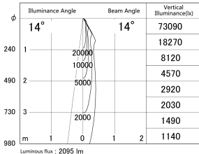
■ Direct Horizontal Illuminance DD139-2015MW9027D
