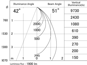
■ Direct Horizontal Illuminance DD139-2050MW9027D
