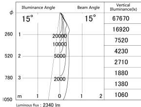
■ Direct Horizontal Illuminance DD139-2515MW9027D
