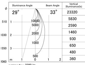
■ Direct Horizontal Illuminance DD139-2530MW9027D
