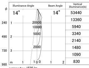
■ Direct Horizontal Illuminance DD139-1515MW9030D
