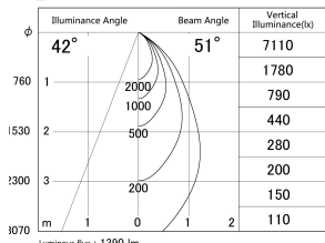
■ Direct Horizontal Illuminance DD139-1550MW9030D
