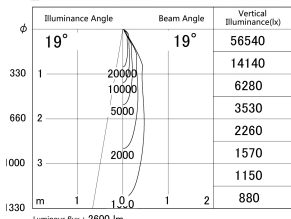
■ Direct Horizontal Illuminance DD139-2520MW9030D
